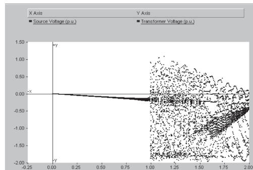
Fig. 13 The bifurcation diagram of transformer voltage with respect to the change in supply voltage
