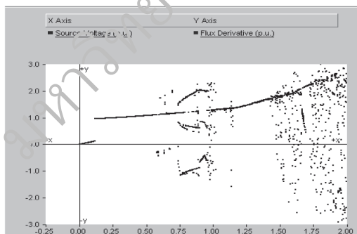
Fig. 10 The bifurcation diagram with PSCAD/EMTDC and Multiple Poincaré Map for single-phase ferroresonant circuit
