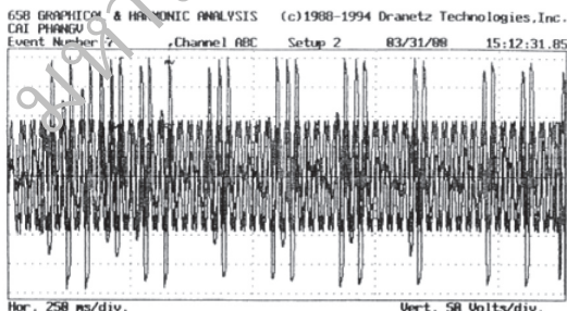
Fig. 12 The oscilogram of the field test after de-energization of phase A
