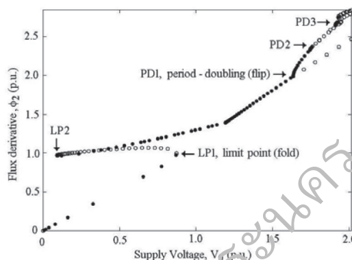
Fig. 2 The steady-state bifurcation diagram generated by the continuation technique with zero initial conditions
