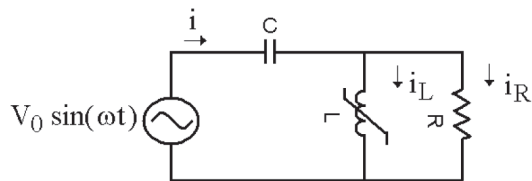
Fig. 1 Simple ferroresonant circuit
